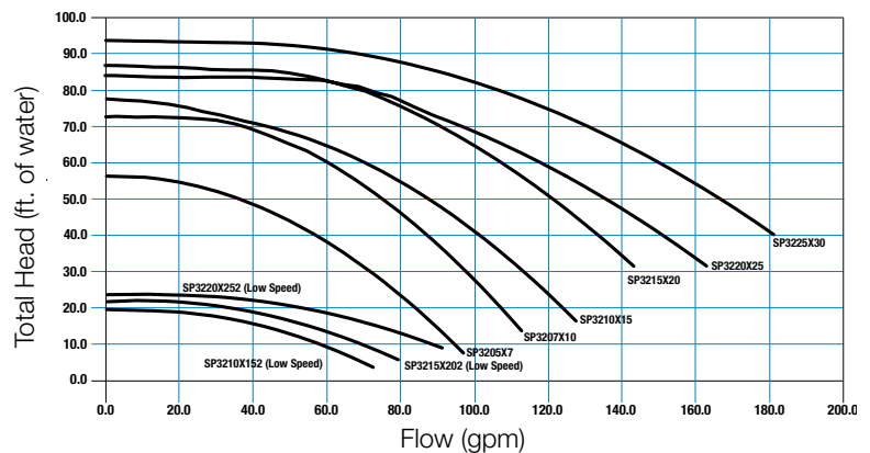
TriStar Standard Efficient Flow vs. Total Head
